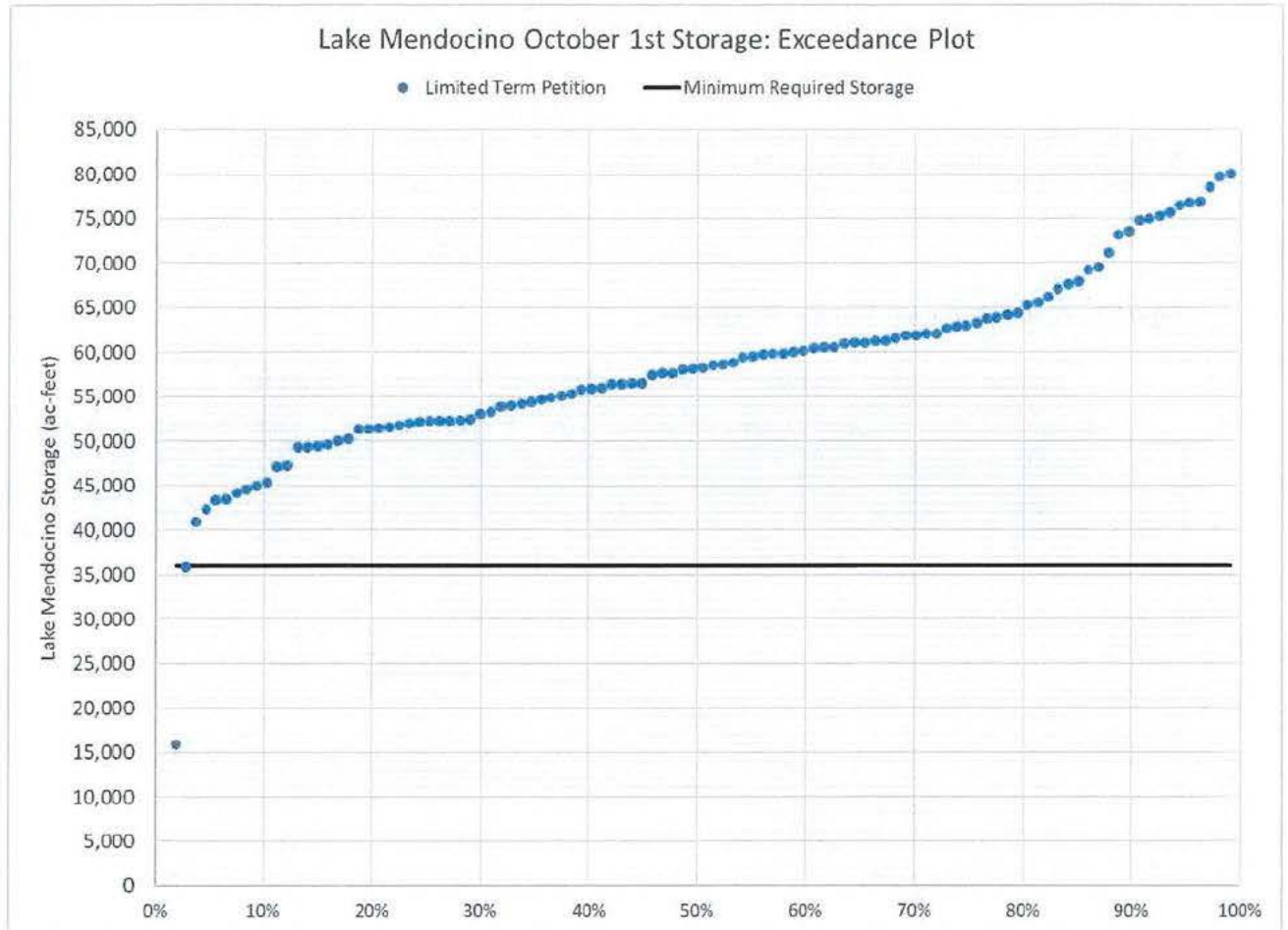
Figure 3: Exceedance Plot of Simulated October 1st Lake Mendocino Storage
